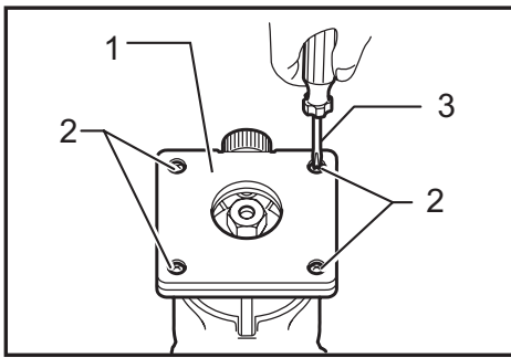
► 1. Base protector 2. Screws 3. Screwdriver
