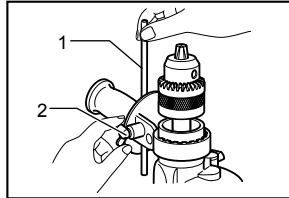
1. Depth gauge 2. Wing nut
