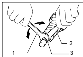
1. Wrench 17 2. Wrench 10 3. Collet nut
