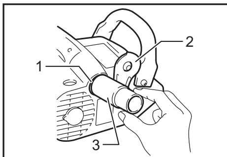
► 1. Dust port 2. Cover plate 3. Joint
