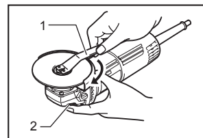
1. Lock nut wrench 2. Shaft lock
